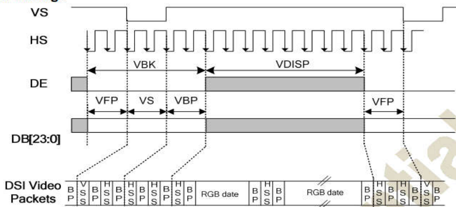
Vertical Timings for DPI I/F
