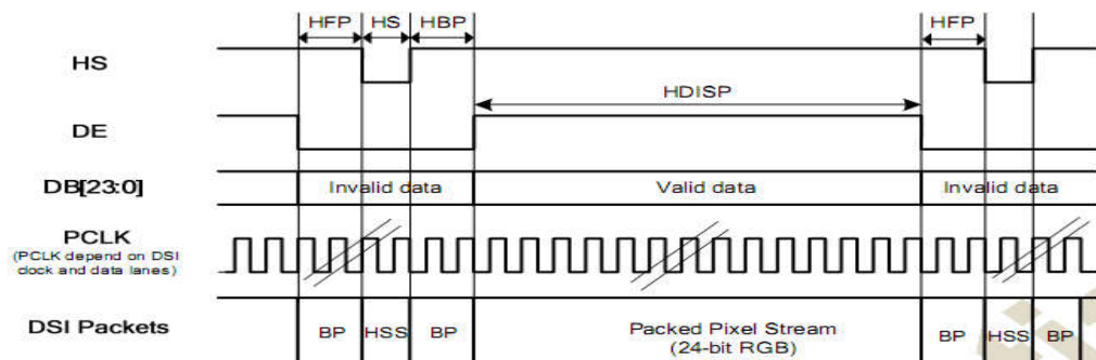
Horizontal Timing for DSI Video mode I/F
